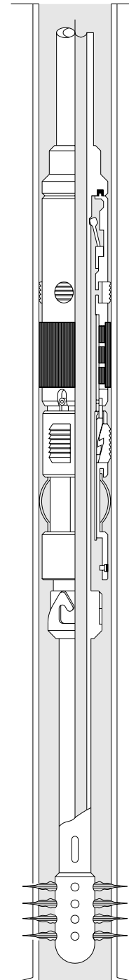
Typical Completion Using the HB-6 Packer
