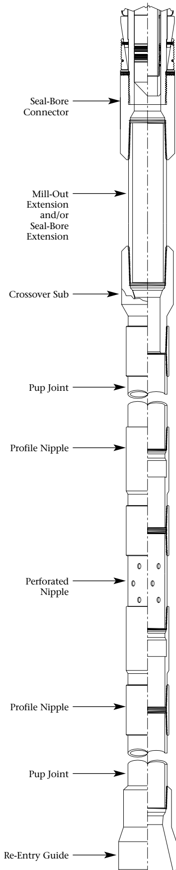
Typical Hookup with Mill-Out Extension, Flow Control Accessory and Re-Entry Guide
