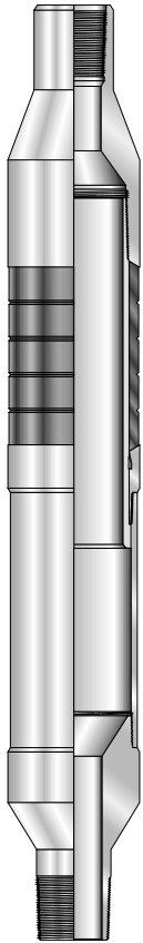
H Pin Packer
